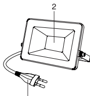
(EU) 1m(3.28ft) H05RN-F 2x1.0mm 2
