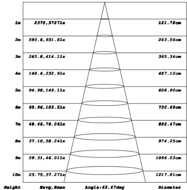
Flux out: 2913 lm
