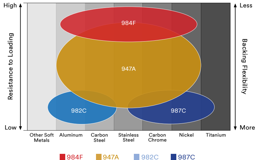
Our new lineup for 3M™ Cubitron™ II Abrasive Discs
