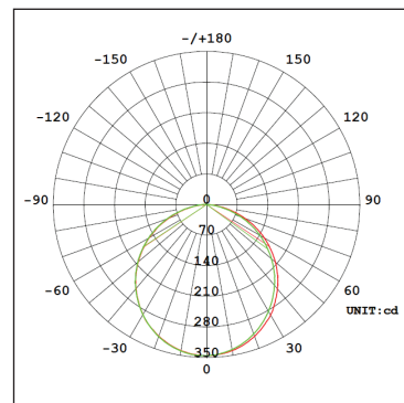
(27W) Lumen Output: 800 - 1040lm
