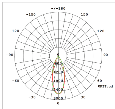
(18W) Lumen Output: 1010 - 1260lm
