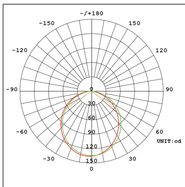
(9W) Lumen Output: 285 - 350lm
