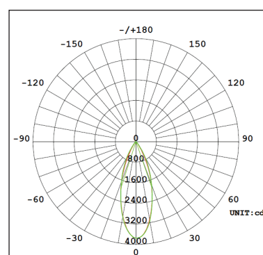
(27W) Lumen Output: 1440 - 1900lm
