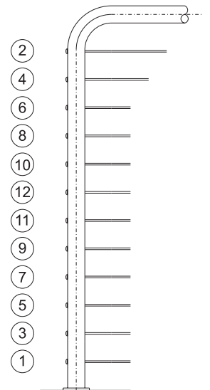
RECOMMENDED TENSIONING SEQUENCE
