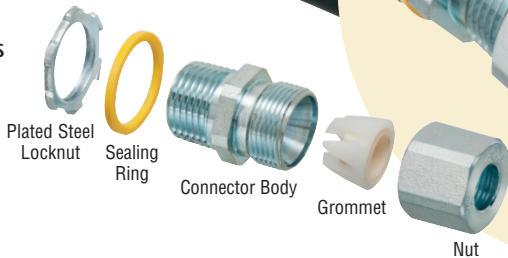
Steel LPCG50S Exploded View
