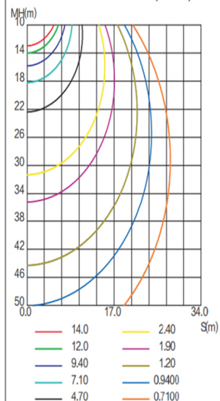
CO PLANE ISOLUX DIAGRAM (UNIT:lx)
