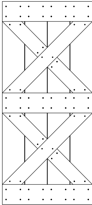
FRONT VIEW (DOUBLE X-BRACE SHOWN)
