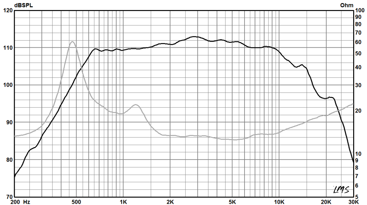
Frequency response and impedance of 760PB-16 on specified horn, free field 3 .
