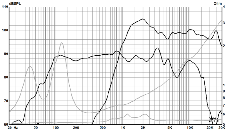
Frequency response and impedance of 6CRS5130-R individual drive units in V_b=6.5 L/ F_b=65 Hz vented box, free field.
