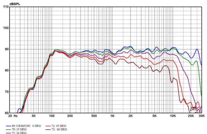
Directivity response curves of CRS6530C with recommended XO in V_b=6.5 L/ F_b=65 Hz vented box, free field.
