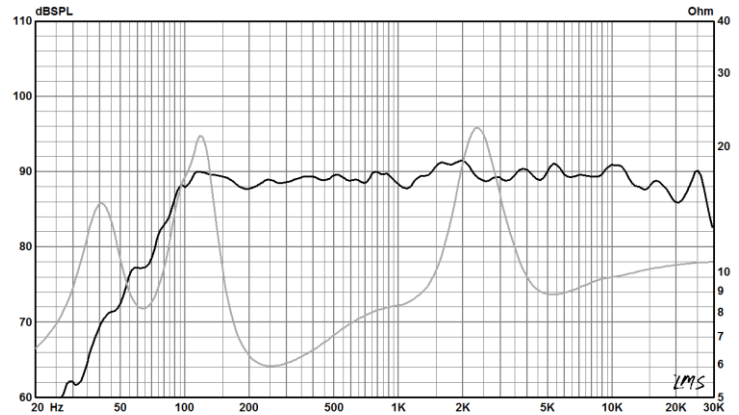
Combined frequency response and impedance of 6CRS5130-R with recommended XO in V_b=6.5 L/ F_b=65 Hz vented box, free field.
