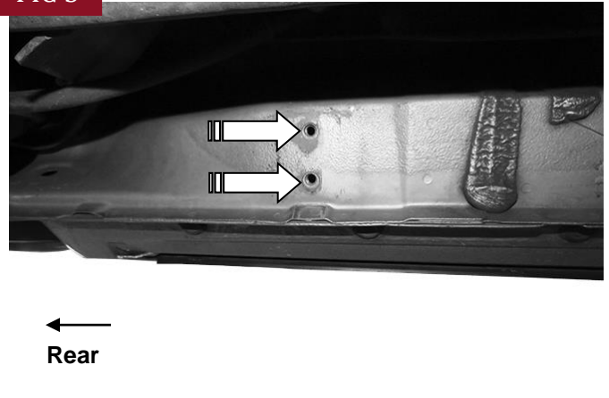
(Fig 5) Driver/Left Rear mounting location
