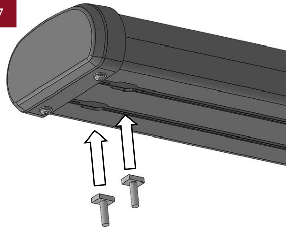
(Fig 7) Insert (6) 6mm T-Bolts into the channels in the bottom of the Side Step, (3 T-Bolts per channel)
