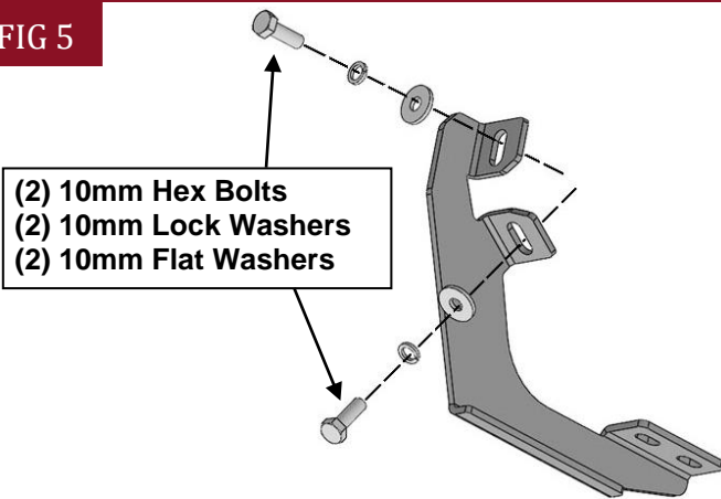
(Fig 5) Attach (1) Center Mounting Bracket to the center location
