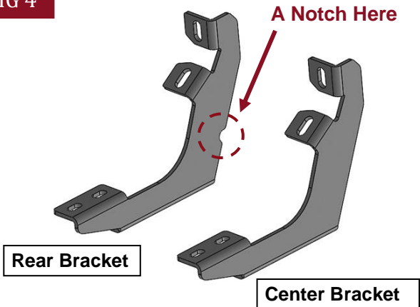
(Fig 4) The Center and Rear Mounting Brackets are similar but unique. The Rear Mounting Bracket has a notch in the back
