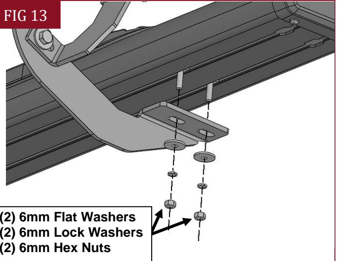
(Fig 13) Attach the Driver/Left Side Step to the (3) Mounting Brackets
