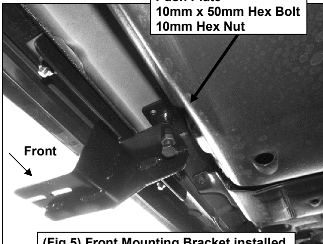
(Fig 5) Front Mounting Bracket installed
