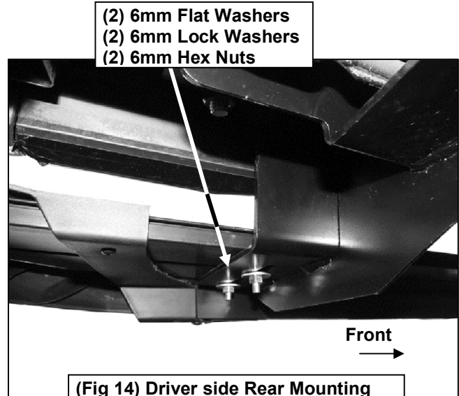
(Fig 14) Driver side Rear Mounting Bracket attached to Running Board
