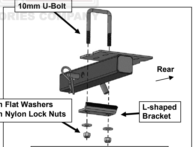
(Fig 4) Attach the L Bracket to the bottom of the Draw Bar and up against the hitch to prevent rattling
