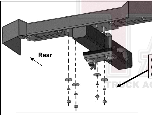
(Fig 8) Attach Board to Draw Bar Plate
