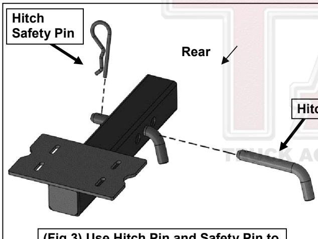
(Fig 3) Use Hitch Pin and Safety Pin to secure the Draw Bar into the hitch
