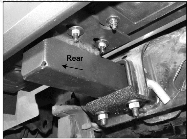
(Fig 9) Rear Step attached to Draw Bar
