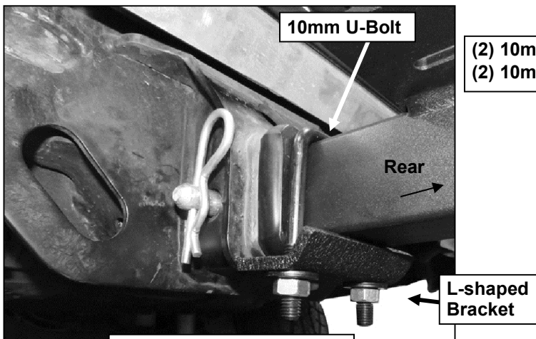
(Fig 5) L Bracket installed
