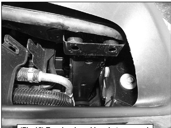
(Fig 15) Tow hook and bracket removed
