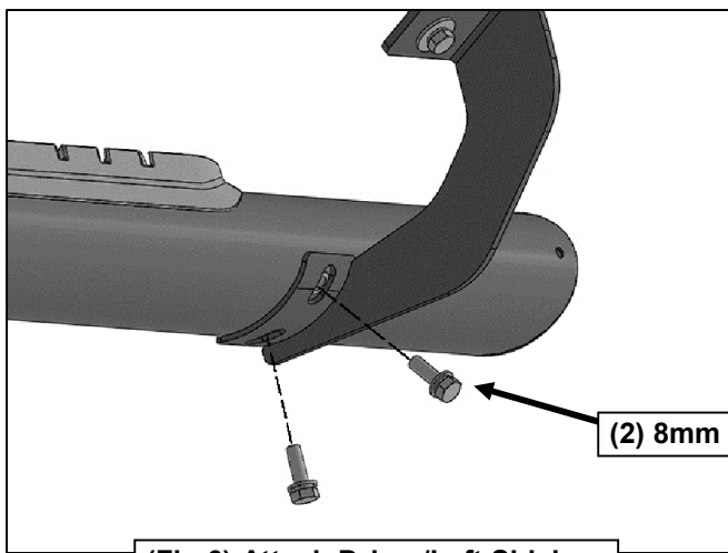
(Fig 6) Attach Driver/Left Sidebar to the Front Mounting Bracket
