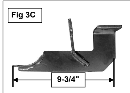
(Fig 3C) Passenger side "long" center Bracket pictured
