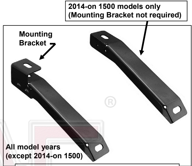
(Fig 3A) Driver/left Center Bracket assembly
