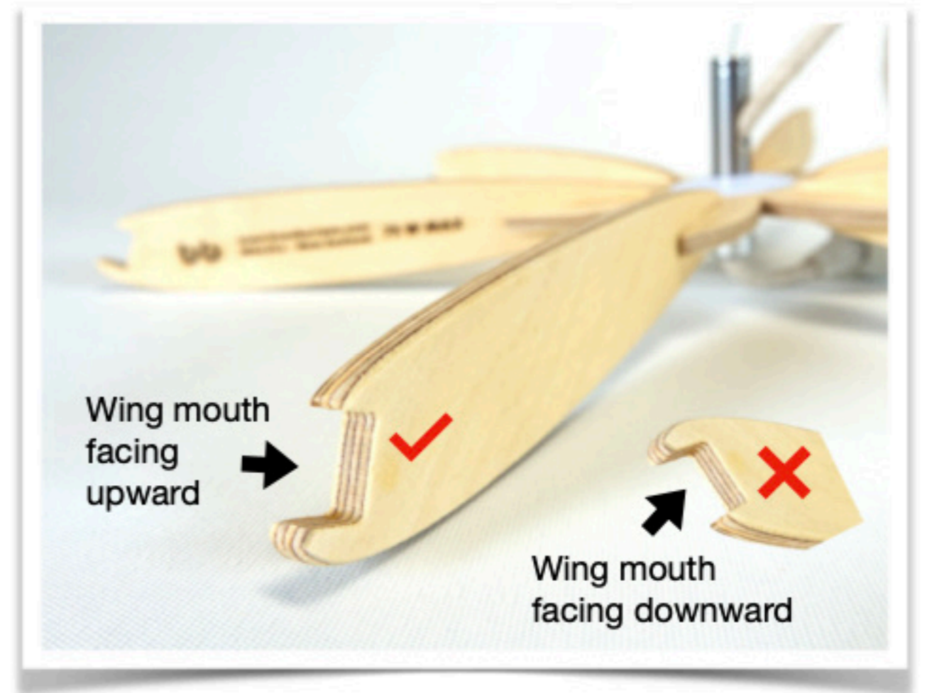
Ensure wing mouths face upward .
