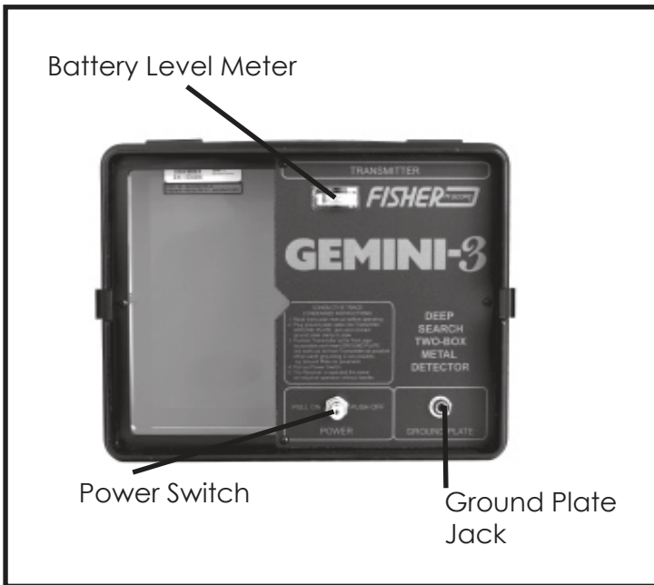
Figure 2. Transmitter
