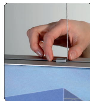
LAGOON PROFILE
