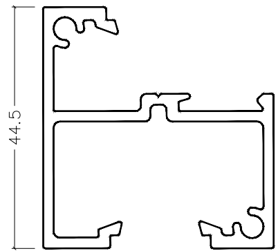
CI-5029 Narrow Midrail
