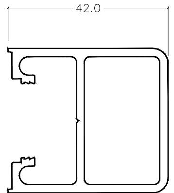
CI-6048 Slimline Plain Stile
