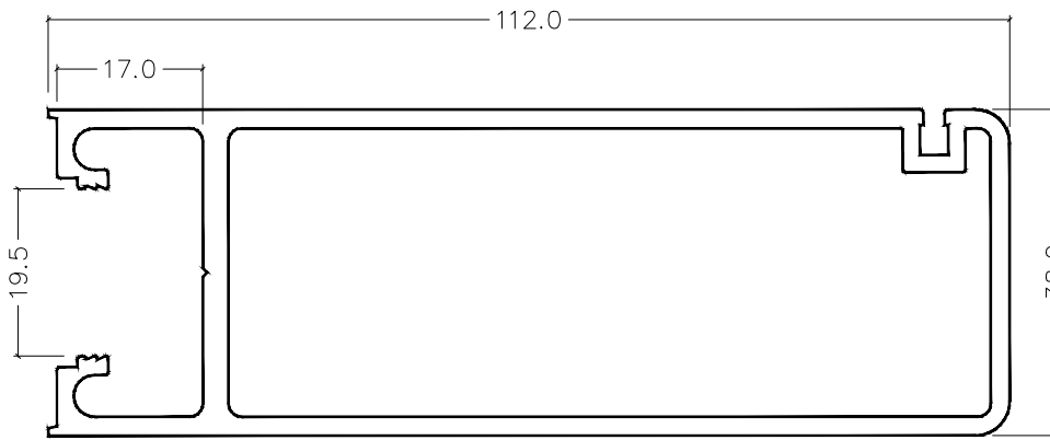
CI-6036 Wide Wiper Stile
