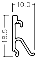
CI-S7556 Sill Bead for 75 mm Sill
