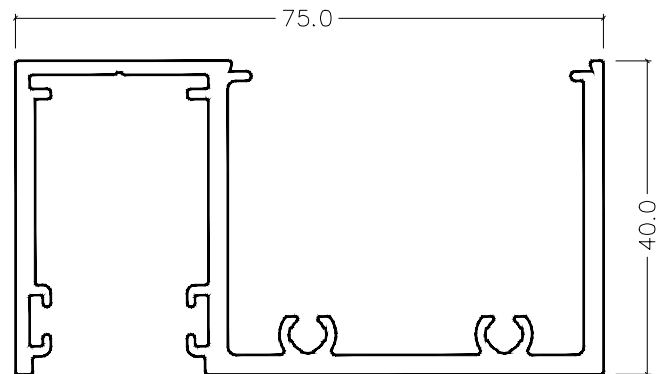
CI-S7554 (CI-S0654) Window Frame
