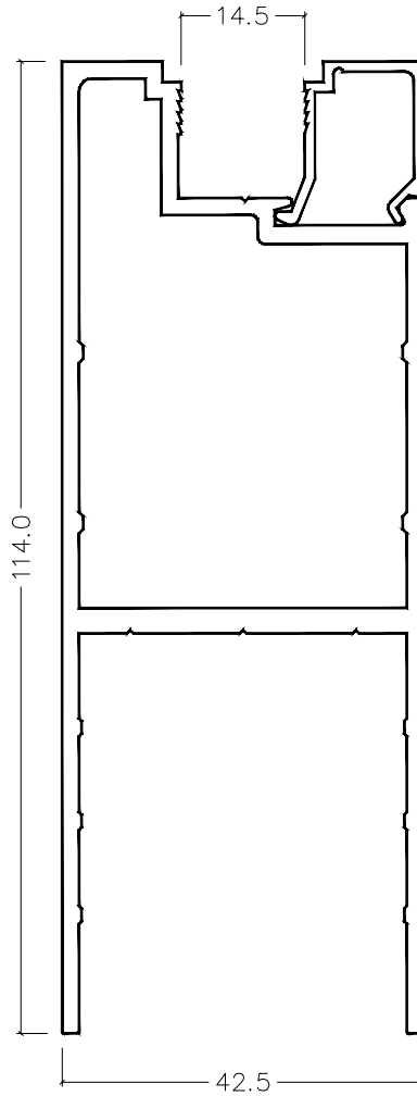
CI-5024 Wide Rail
