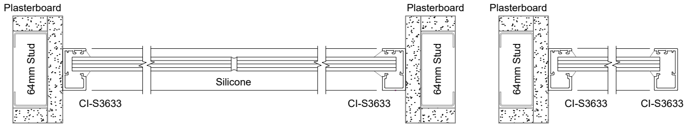
SVELTE 36 Single Glaze
