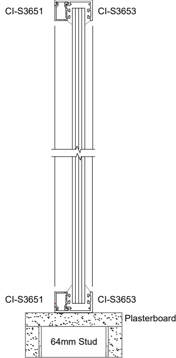
SVELTE 36 Slimline Single Glaze Half Wall
