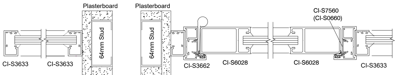
SVELTE 36 Single Glaze Side Light with Aluminium Hinged Door
