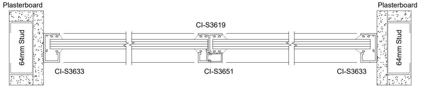
SVELTE 36 Single Glaze with Midrail
