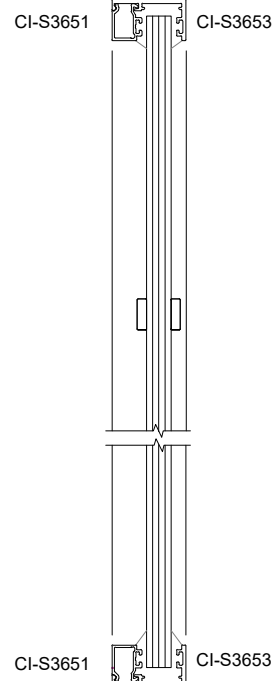
SVELTE 36 Slimline Single Glaze with Back to Back
