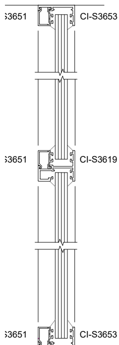
SVELTE 36 Slimline Single Glaze with Mid rail
