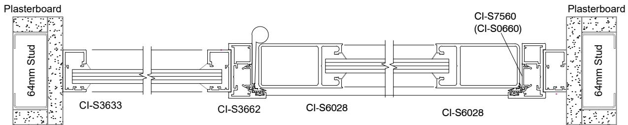
SVELTE 36 Single Glaze Sidelight and Aluminium Door
