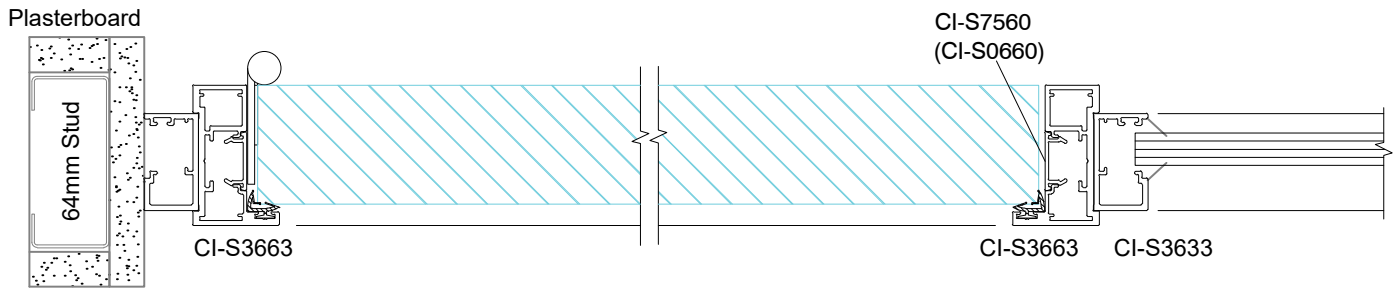
SVELTE 36 Single Glaze Side Light and Timber Door 44 mm
