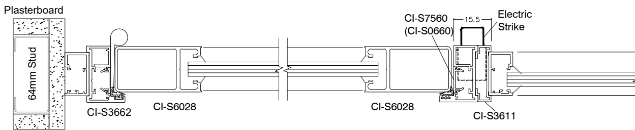
SVELTE 36 Single Glaze Side Light with Aluminium Door + Door Jamb Spacer for Electric Strike
