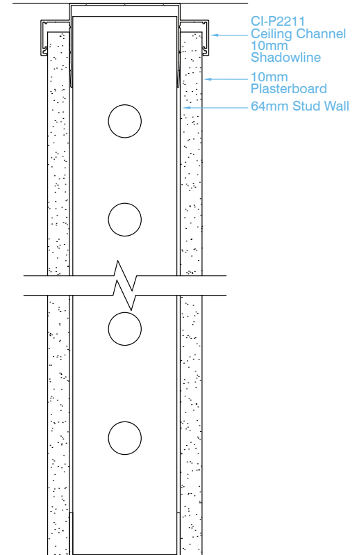
Platinum 90 Plaster Wall with Shadowline
