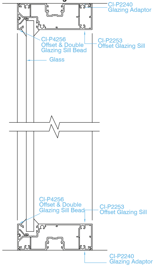
Platinum 90 Double Glaze using Sill Bead
