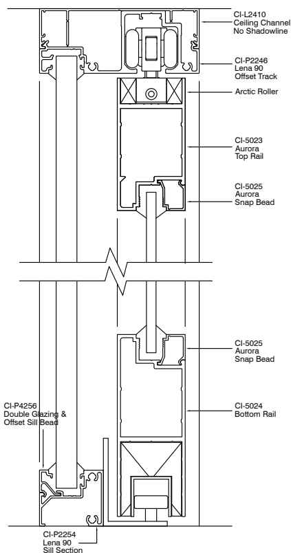
Platinum 90 Offset Glaze with Sliding Door
