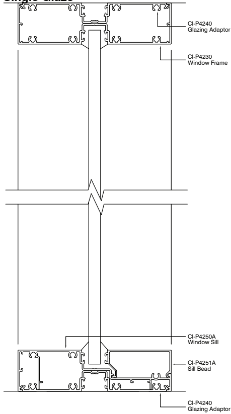
Single Glaze
