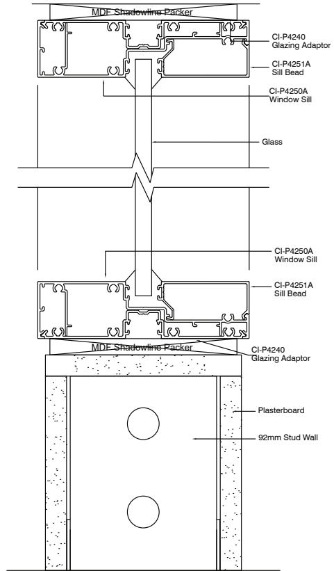
Single Glaze Half Wall
