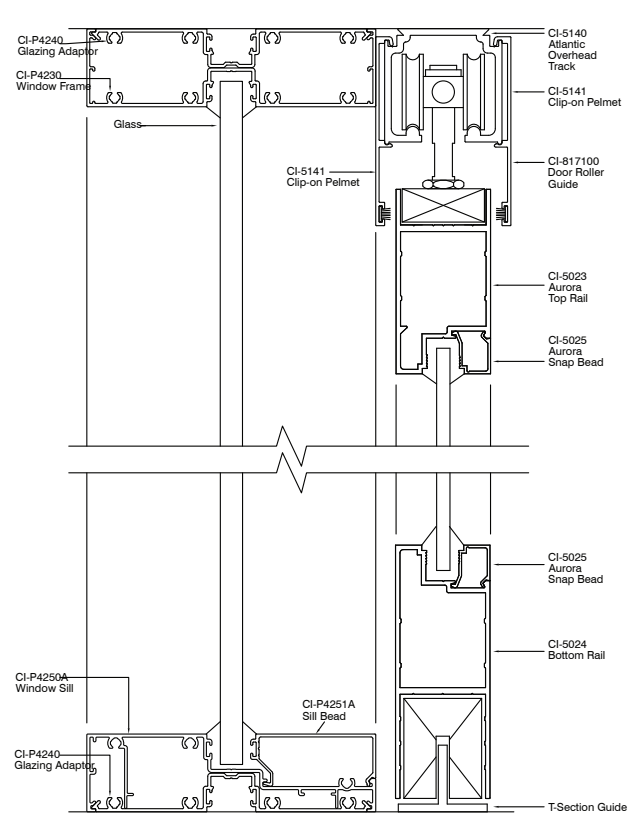
Platinum 120 Single Glaze with Sliding Door
