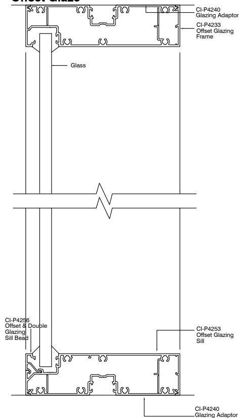
Platinum 120 Offset Glaze
