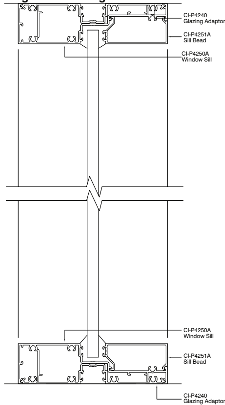
Platinum 120 Single Glaze using Sill Bead
