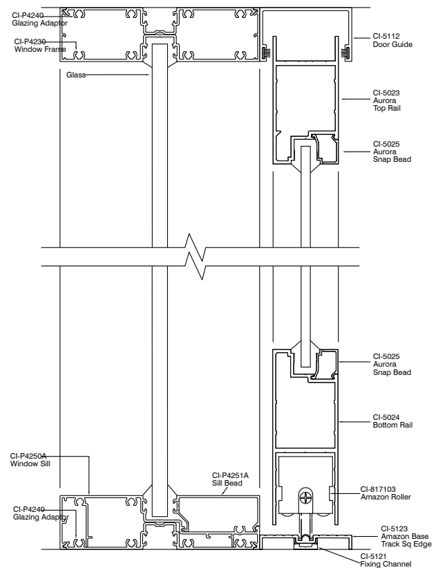
Platinum 120 Single Glaze with Sliding Door Bottom Track
