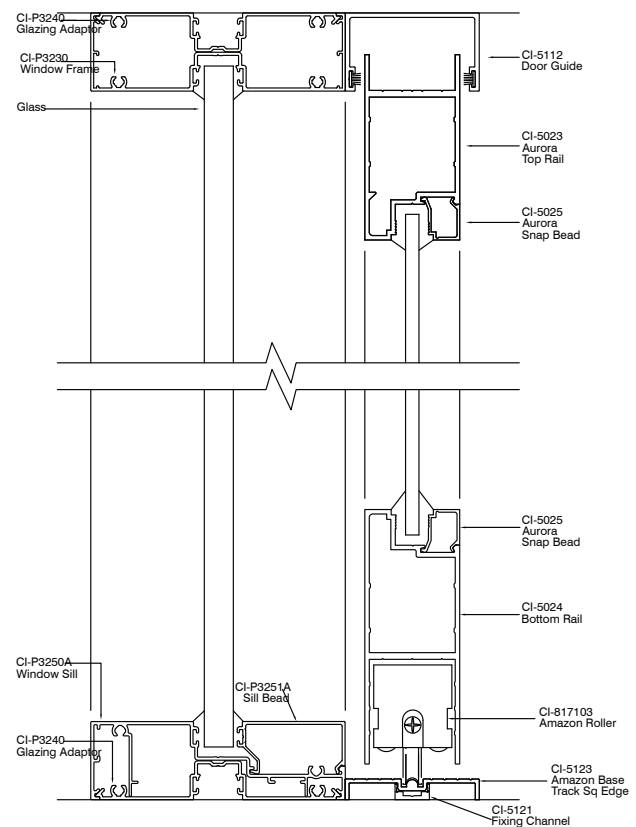
Platinum 105 Single Glaze with Sliding Door Bottom Track
