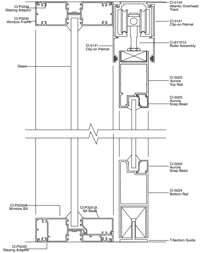
Platinum 105 Single Glaze with Sliding Door Bottom Track
