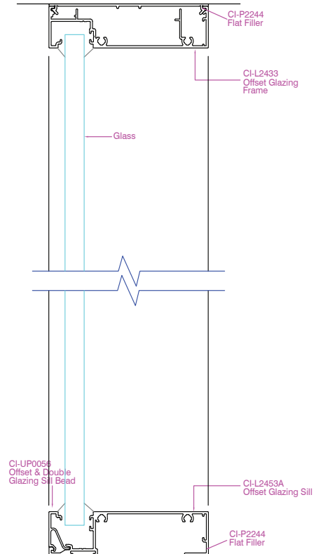
Linium 90 Offset Glaze
