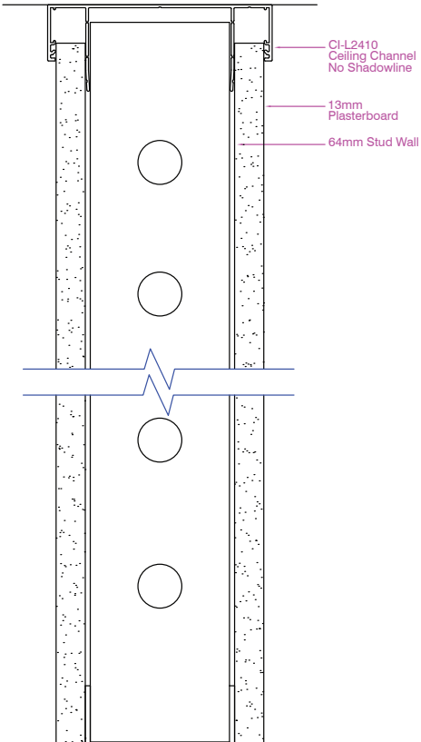
Linium 90 Plaster Wall with no Shadowline
