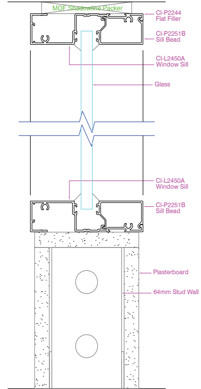
Linium 90 Single Glaze
