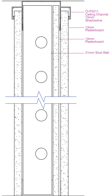
Linium 90 Double Plaster Wall with Shadowline
