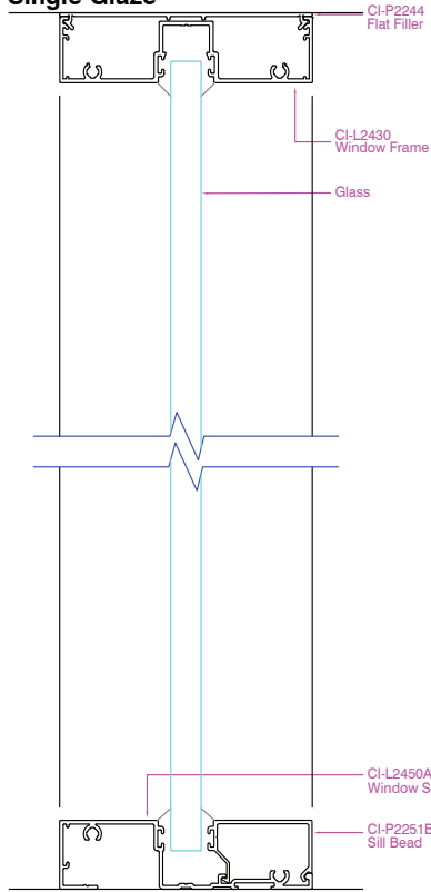
Linium 90 Single Glaze
