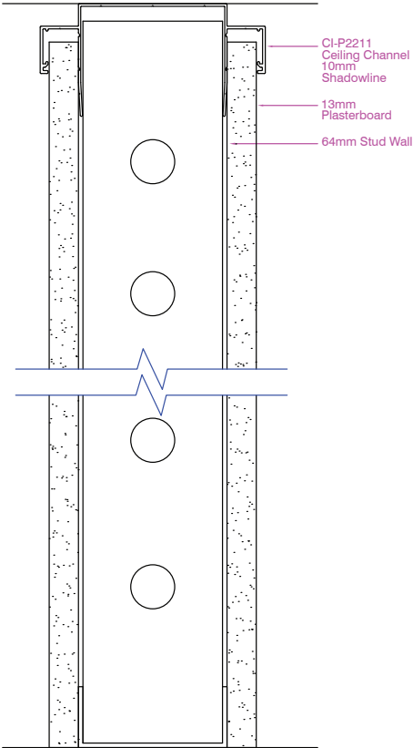
Linium 90 Plaster Wall with Shadowline
