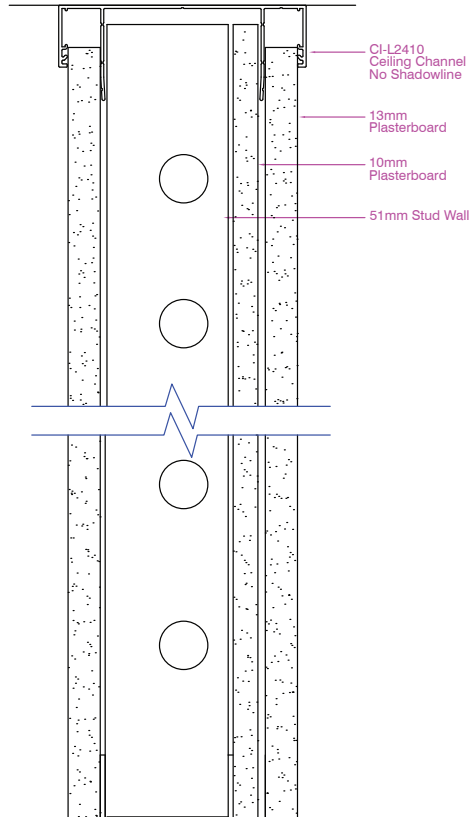
Linium 90 Double Plaster Wall with no Shadowline
