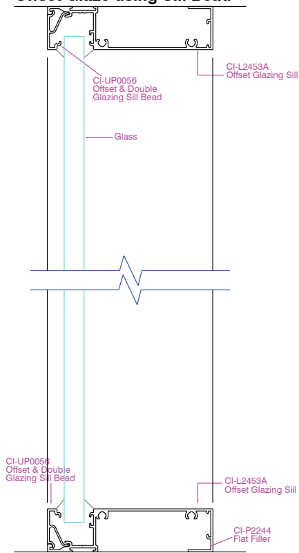
Linium 90 Offset Glaze using Sill Bead
