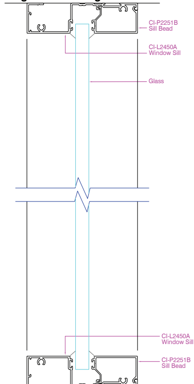
Linium 90 Single Glaze using Sill Bead
