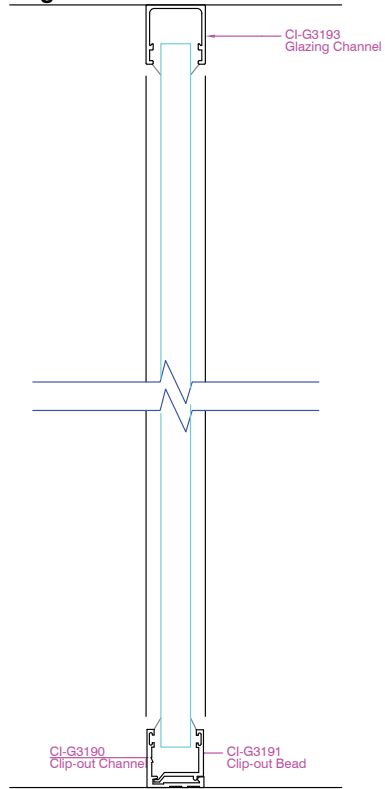
Gallium 25 Glazing Frame
