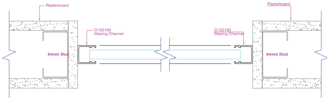
Gallium 25 Glazing Frame
