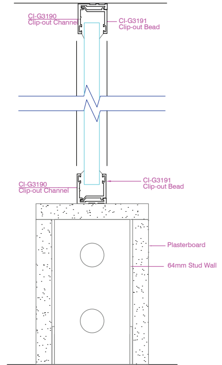
Gallium 25 Glazing Frame Half Wall
