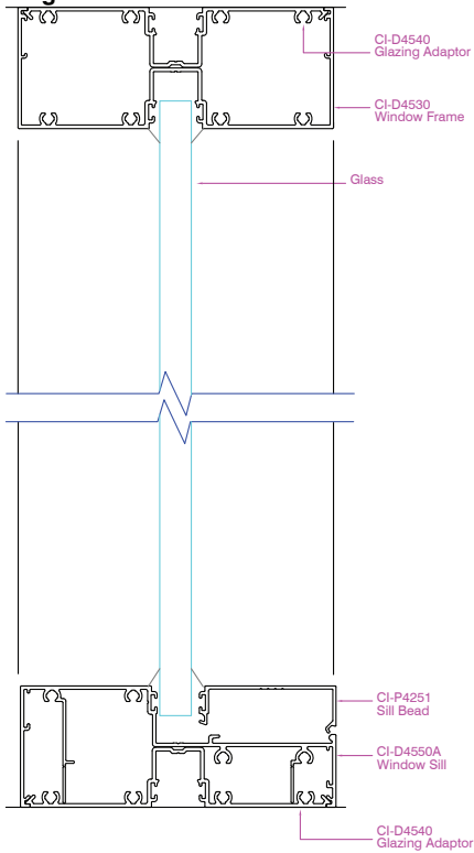
Definium 120 Single Glaze
