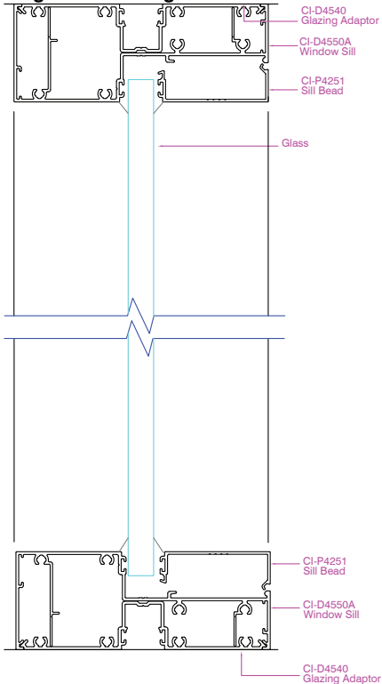
Definium 120 Single Glaze using Sill Bead
