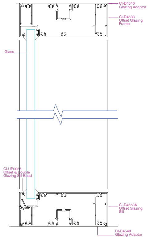
Definium 120 Offset Glaze
