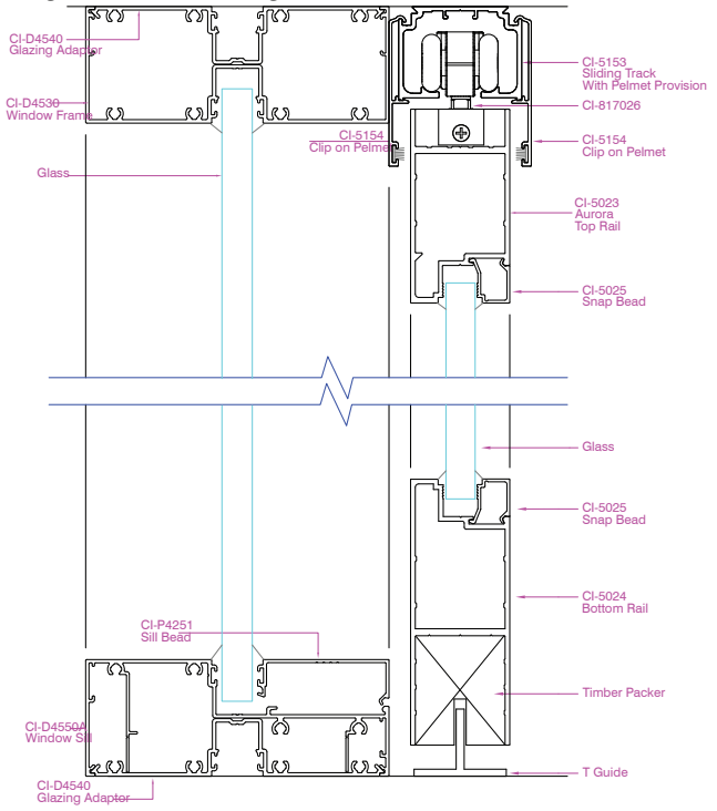
Definium 120 Single Glaze with Sliding Door
