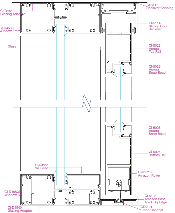
Definium 120 Single Glaze with Sliding Door Bottom Track
