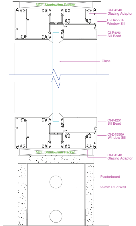
Definium 120 Single Glaze Half Wall
