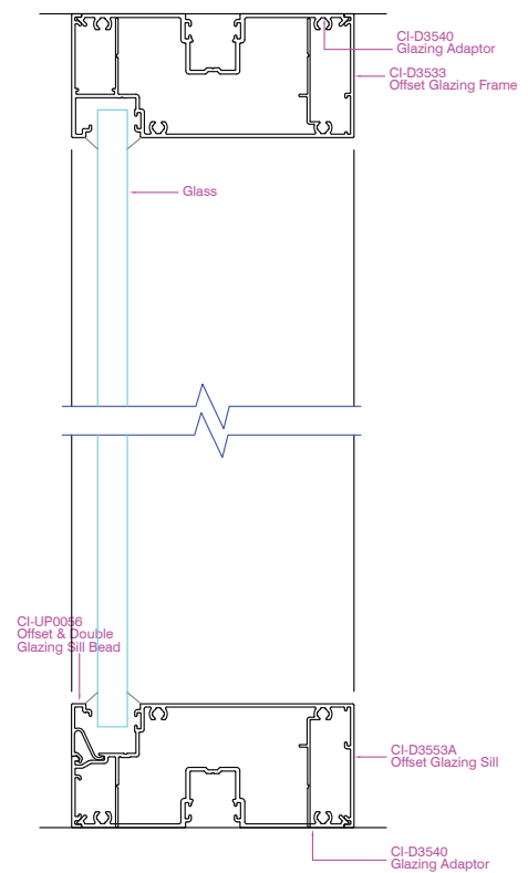
Definium 105 Offset Glaze
