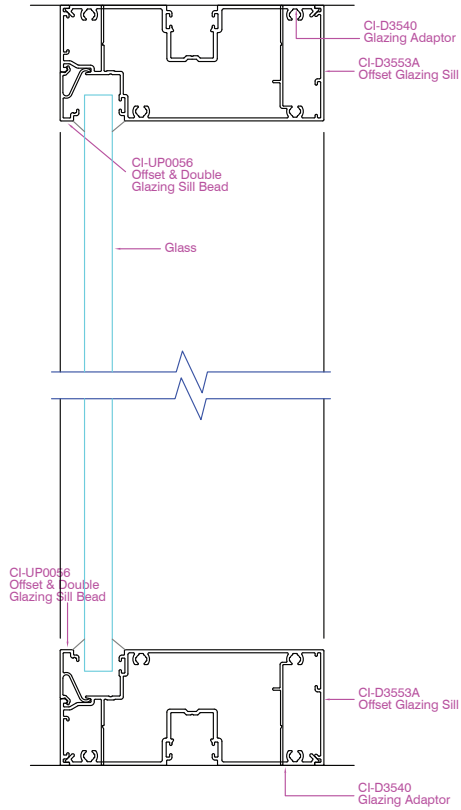
Definium 105 Offset Glaze using Sill Bead
