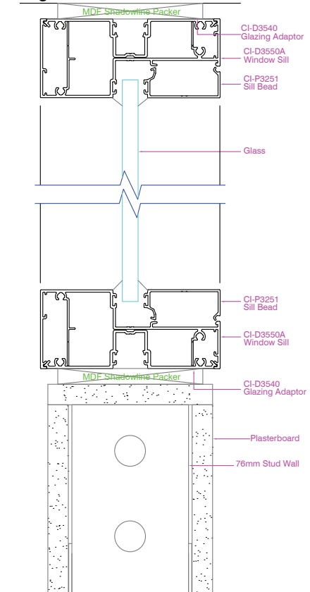
Definium 105 Offset Glaze
