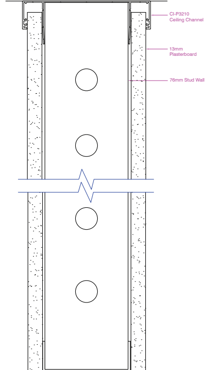
Definium 105 Plaster Wall with no Shadowline
