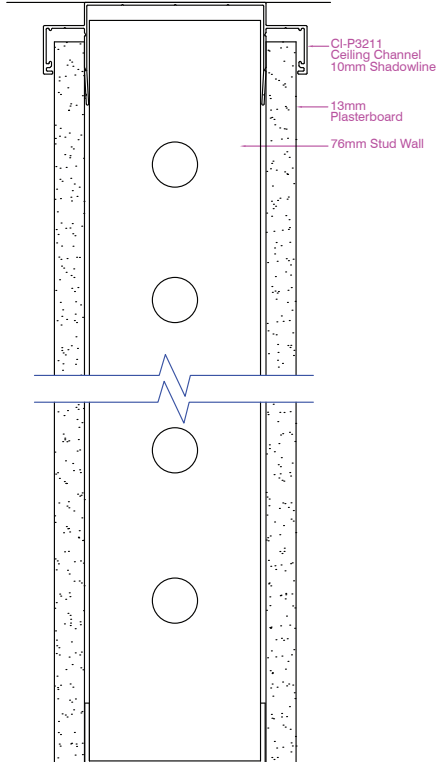
Definium 105 Plaster Wall with Shadowline
