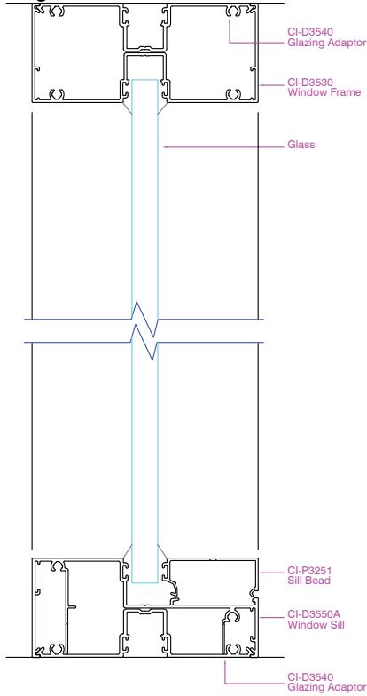
Definium 105 Single Glaze
