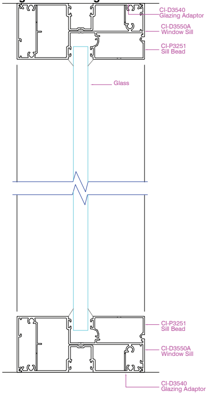
Definium 105 Single Glaze using Sill Bead
