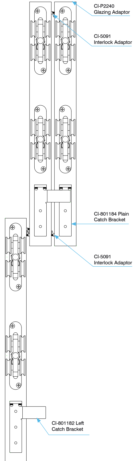
PLAN VIEW
