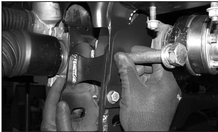
FIGURE 23 - STEP 20
