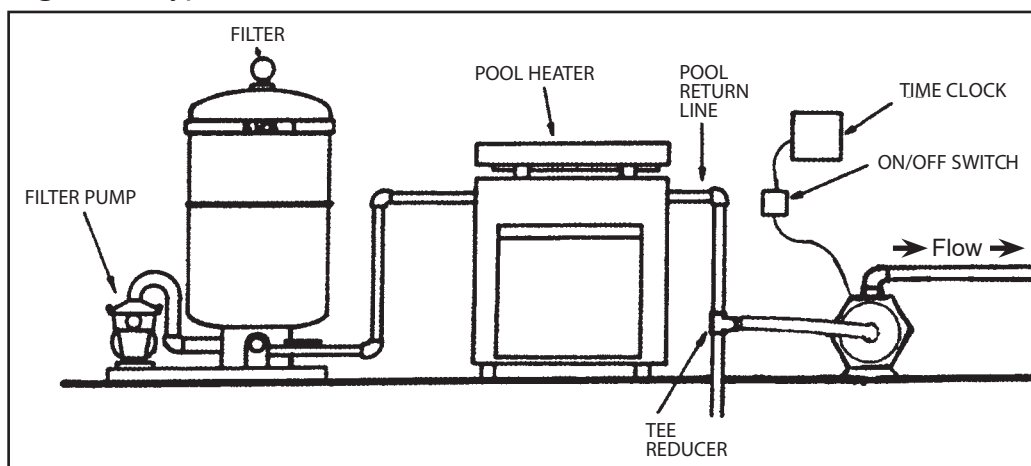
Figure 1: Typical Installation
