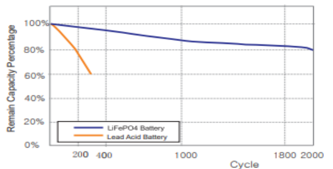
Cycle Life Performance Curve@25°C
