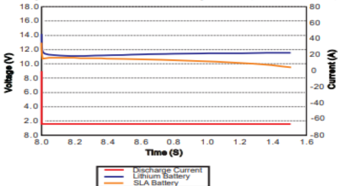
Voltage Vs Time Vs Current Discharge Curve (10 C, 90S, -10°C)
