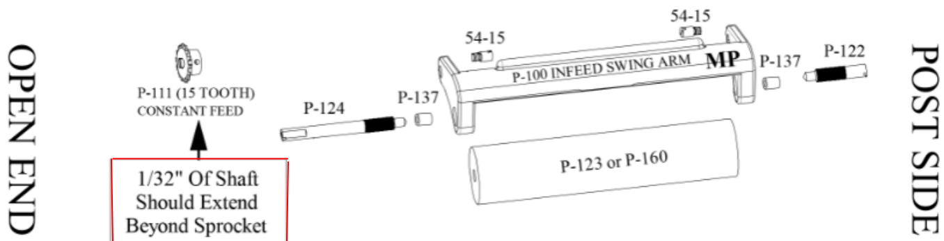
54-513 MULTI-PASS INFEED SWING ARM ASSEMBLY
