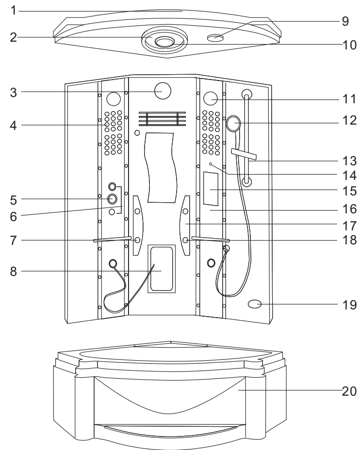
CONSTRUCTION SKETCH
