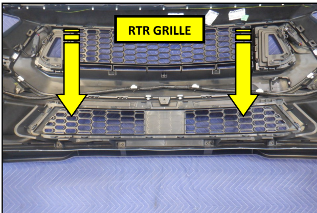
19. Align the bumper cover tabs with the slots in the RTR Grille. Install the RTR Grille onto the bumper cover by engaging the locking tabs, one by one, from left to right.
