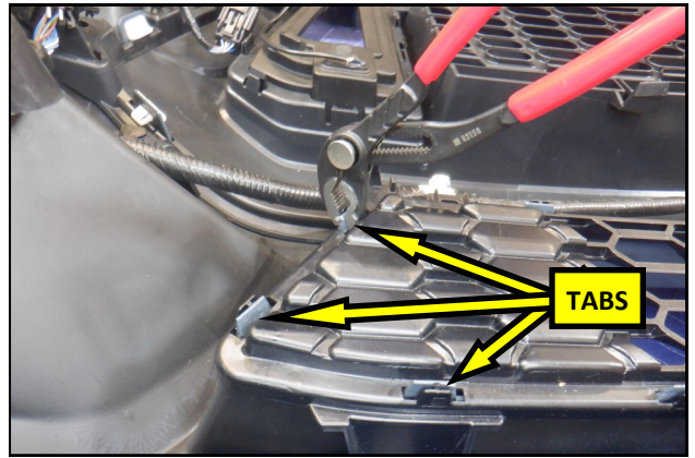
18. Using a pair of slip joint pliers, depress the lower grille locking tabs one by one, from left to right, and remove the OEM grille.
