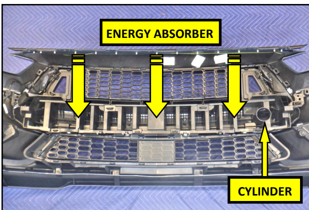
21. Reinstall the energy absorber into the bumper cover as shown.
