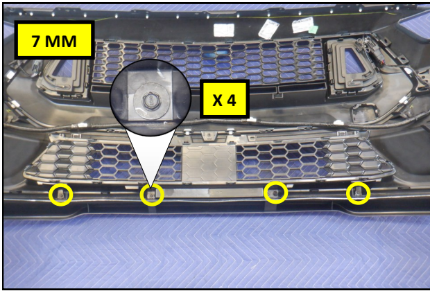
17. Using a 7 mm socket, remove the 4 screws securing the bottom of the lower grille to the bumper cover.
