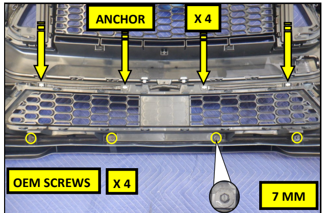
20. Reinsert the harness anchors from step 16 into the RTR Grille. Secure the Grille to the bumper cover using the screws removed in step 17.
