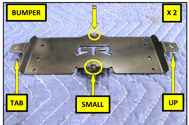
4. Place the Base Plate on a padded work surface as shown, with the mounting tabs raised. Carefully insert the Rubber Bumpers into the Mount, small side first.
