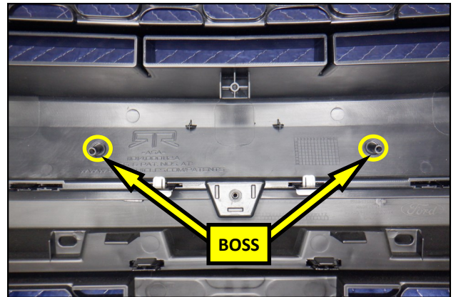
2. Locate the two Screw Bosses in the center of the RTR Grille.
