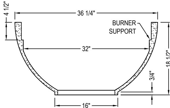
SECTION VIEW
