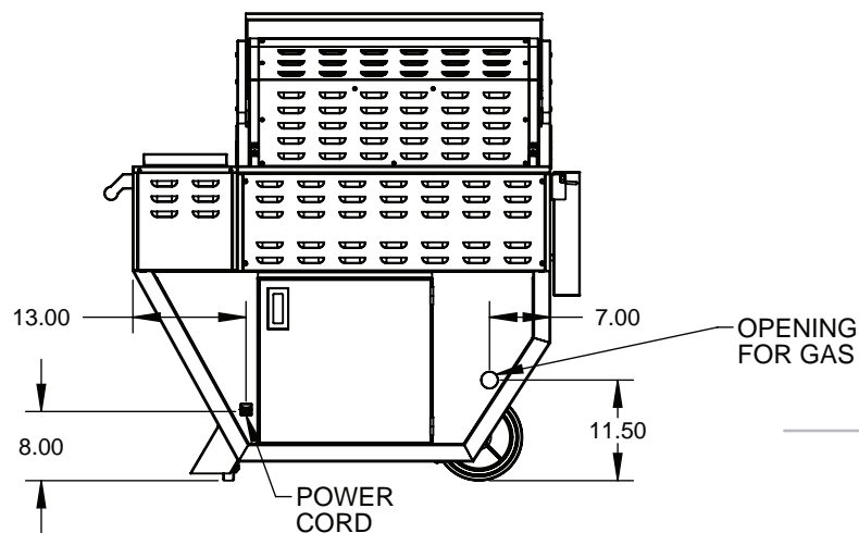
36" REAR VIEW
