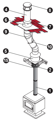
Attic Offset
