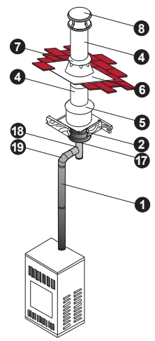
Oil Furnace
