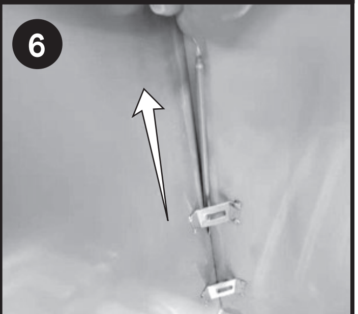
6 Remove oil capillary.
