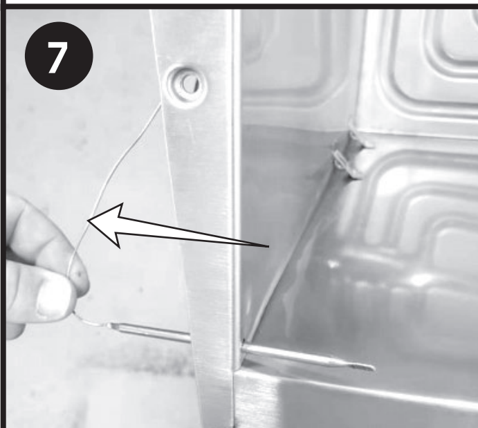
7 Remove oil capillary from the pot.
