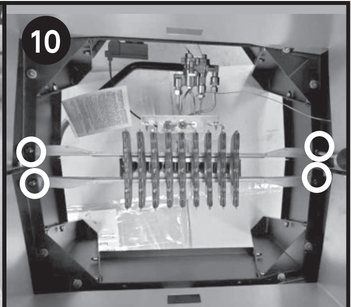
Remove the four (4) Screws holding the bracket.
