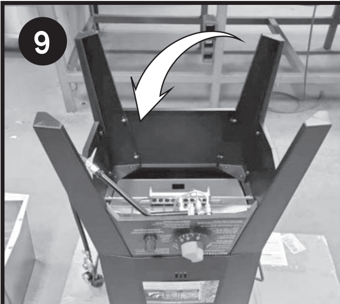
Turn the fryer body upside down.
