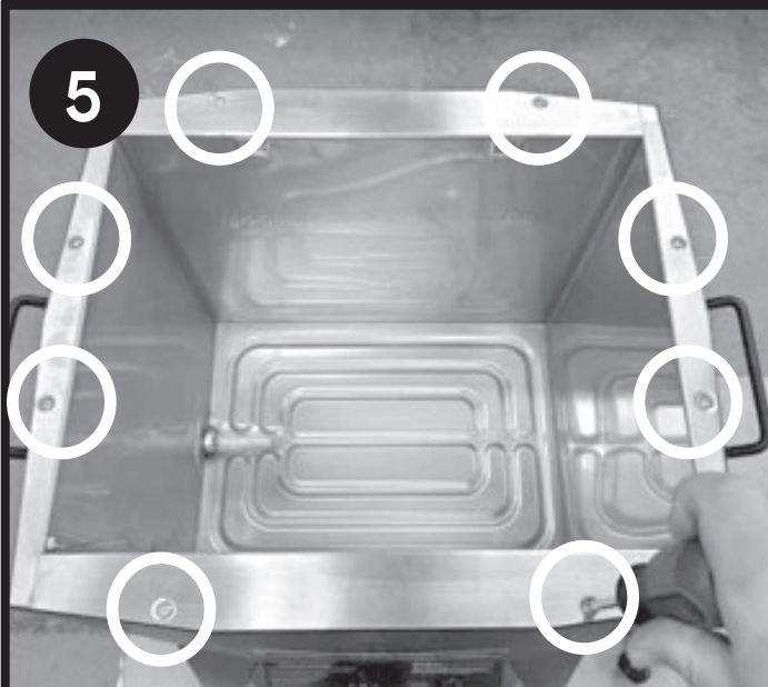
5 Remove eight (8) Screws from the oil pot.
