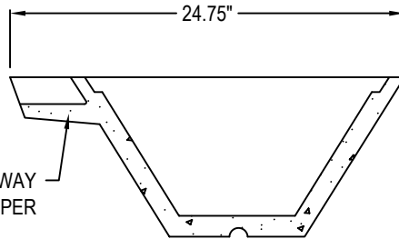
SIDE SECTION
