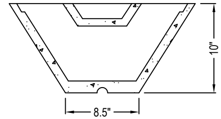
FRONT SECTION
