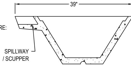
SIDE SECTION
