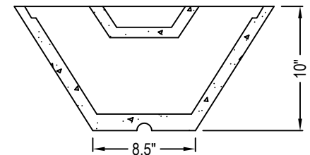
FRONT SECTION
