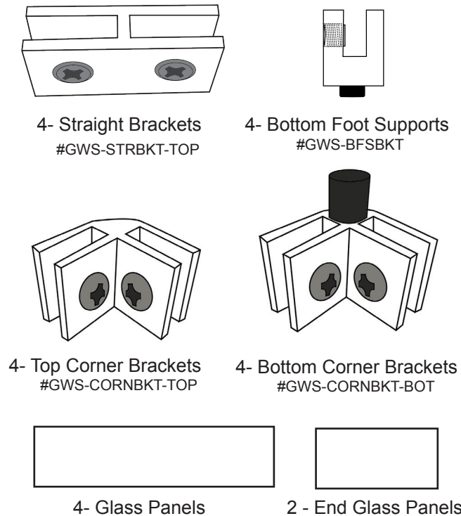
Fig. 1 Shows carton glass panels and rectangular windshield brackets.
