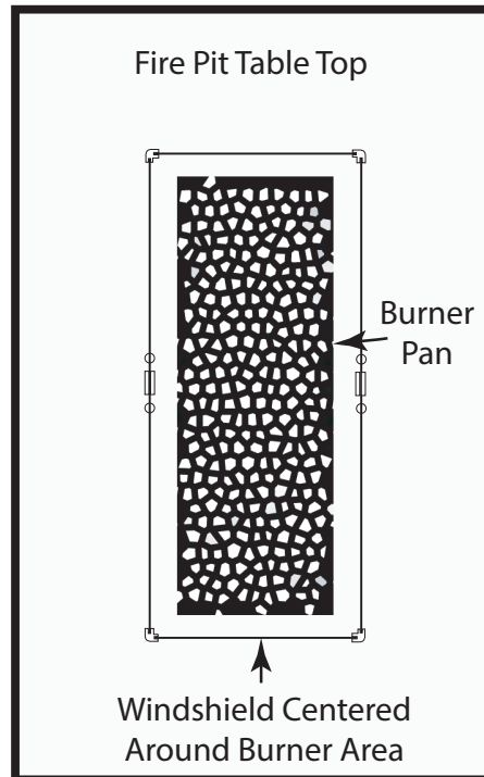
Fig. 6 Windshield installed (top view).
