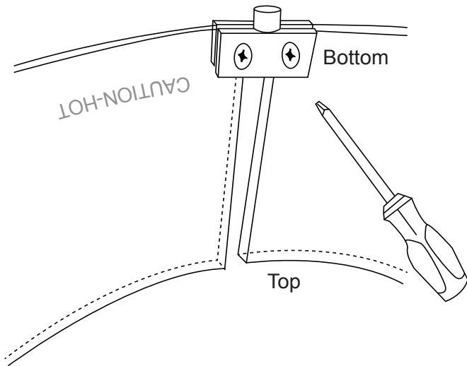
Fig. 7 Securing the brackets screws with a Phillips screwdriver.
