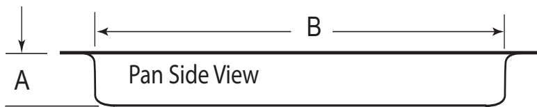
Fig. 1 Fire Pit Dimensions; refer to Table 1. (Dimensions applicable to round or square pans)
