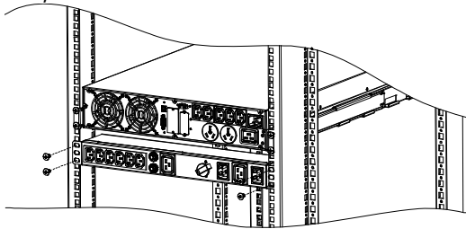
Chart 1: Rack mounting
