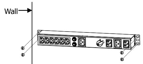
Chart 2: Wall mounting
