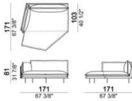
Right or left unit
