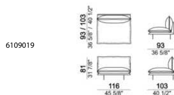
Central unit, back cushion 115 cm.
