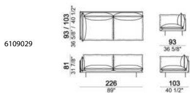
Right or left unit, back cushions 105 cm.
