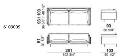
Sofa, back cushions 115 cm
