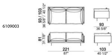
Sofa, back cushions 95 cm
