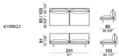
Central unit, back cushions 115 cm.
